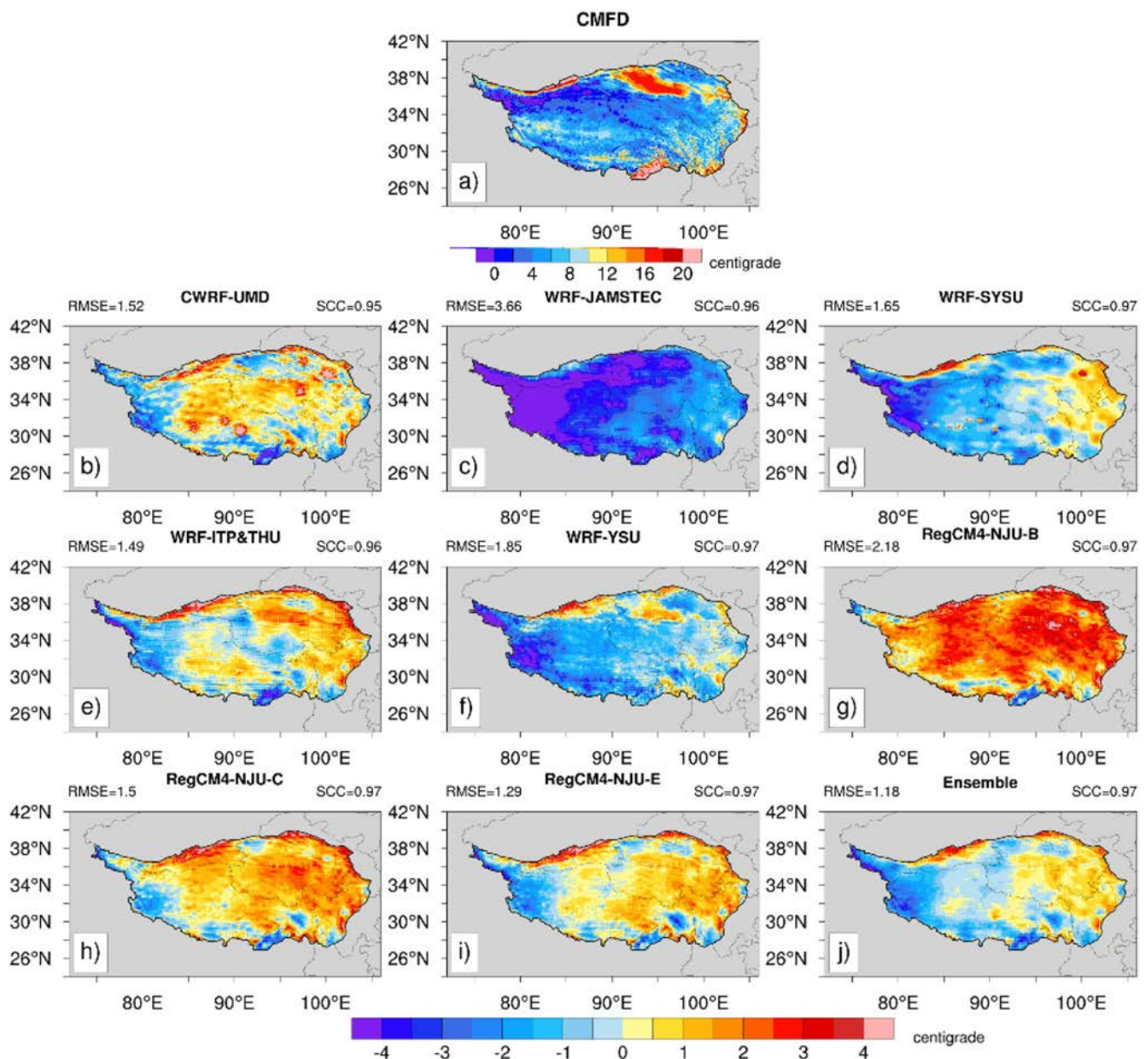
Fig. 5 The MJJA mean temperature at 2-m height ( ^{\circ}\text{C} ) (a–j) over the TP based on the CMFD observation during 1991–2015 (a), and biases of the RCMs (b–i) and multi-model ensemble mean (j)
